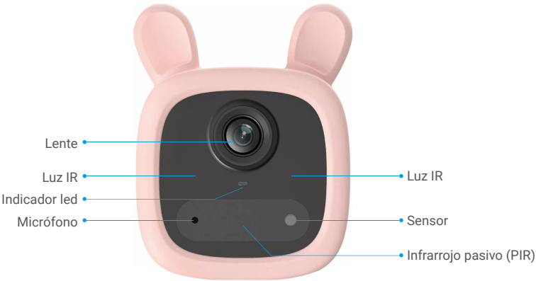
Vista frontal
